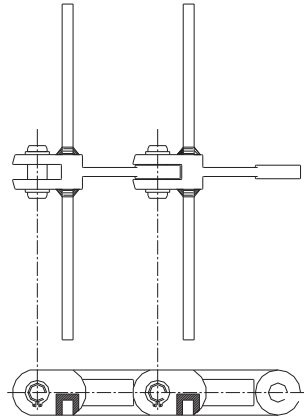
FORGED CHAIN - SQUARE BAR TYPE SCRAPER ATTACHMENTS
